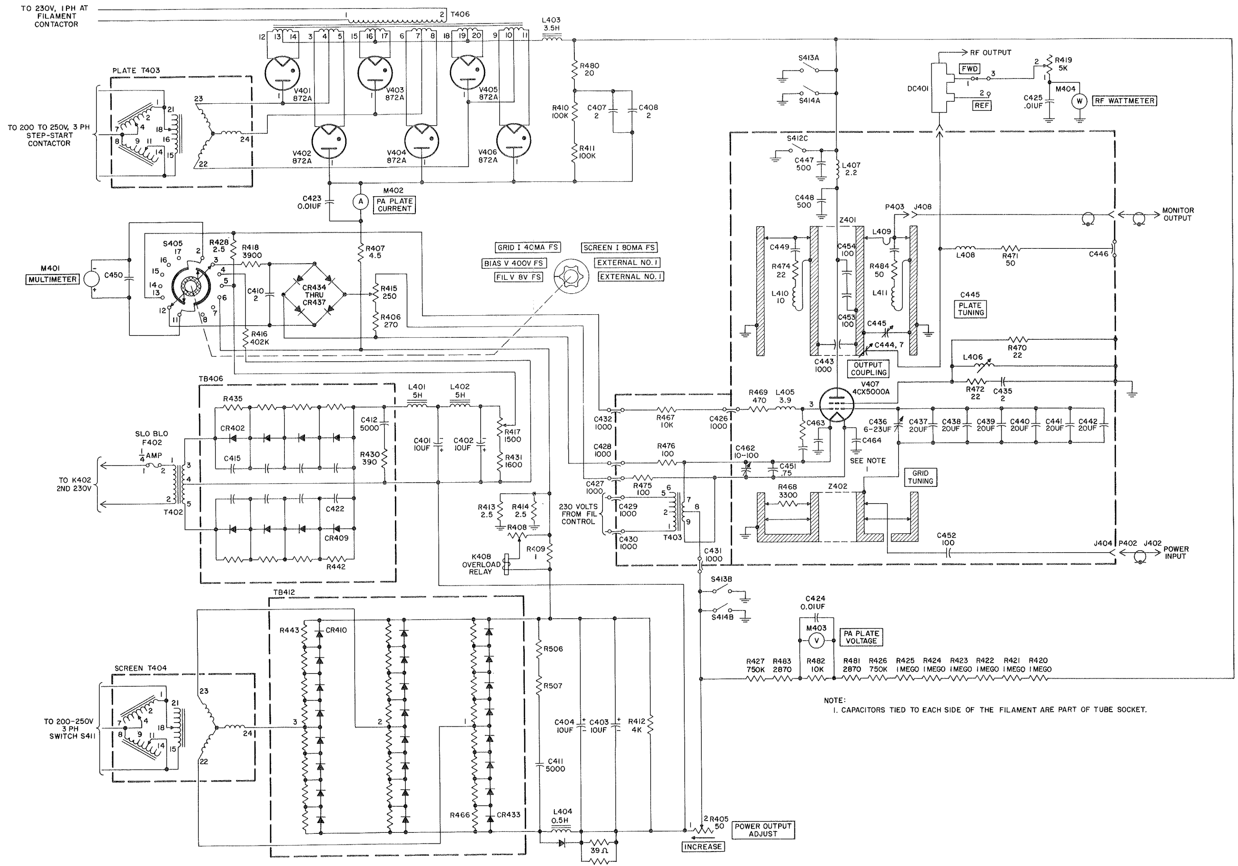
Figure 2-3. E830-1 Power Amplifier Circuits, Simplified Schematic
